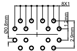
Pcb plate opening size (PCB板开孔尺寸)
