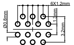
Pcb plate opening size (PCB板开孔尺寸)
