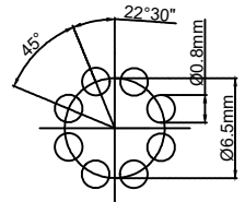
Pcb plate opening size (PCB板开孔尺寸)
