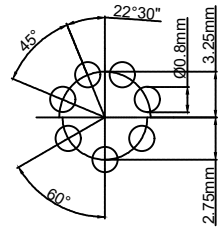
Pcb plate opening size (PCB板开孔尺寸)
