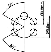
Pcb plate opening size (PCB板开孔尺寸)
