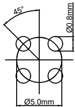
Pcb plate opening size (PCB板开孔尺寸)
