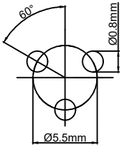
Pcb plate opening size (PCB板开孔尺寸)
