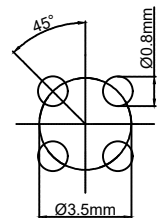
Pcb plate opening size (PCB板开孔尺寸)
