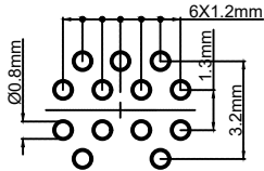
Pcb plate opening size (PCB板开孔尺寸)
