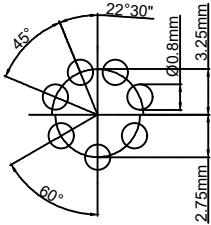
Pcb plate opening size (PCB板开孔尺寸)
