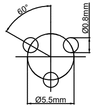
Pcb plate opening size (PCB板开孔尺寸)
