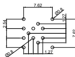
Pcb plate opening size (PCB板开孔尺寸)
