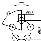
Pcb plate opening size (PCB板开孔尺寸)
