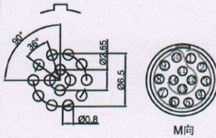
Pcb plate opening size (PCB板开孔尺寸)
