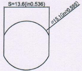
Pane hole size (面板开孔尺寸)
