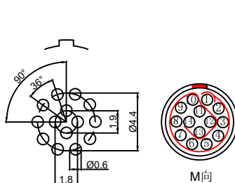
Pcb plate opening size (PCB板开孔尺寸)
