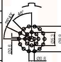
Pcb plate opening size (PCB板开孔尺寸)
