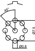
Pcb plate opening size (PCB板开孔尺寸)
