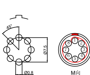
Pcb plate opening size (PCB板开孔尺寸)
