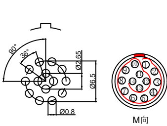
Pcb plate opening size (PCB板开孔尺寸)
