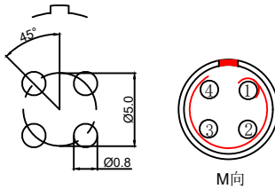
Pcb plate opening size (PCB板开孔尺寸)
