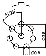
Pcb plate opening size (PCB板开孔尺寸)
