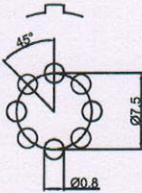
Pcb plate opening size (PCB板开孔尺寸)
