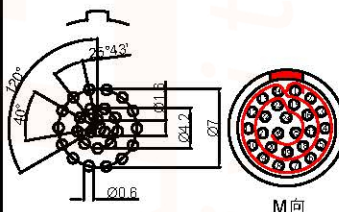
Pcb plate opening size (PCB板开孔尺寸)
