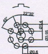
Pcb plate opening size (PCB板开孔尺寸)
