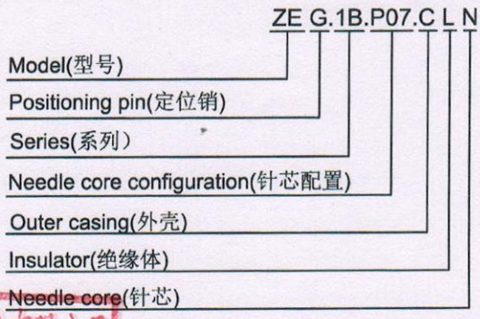
Boarded mother adhesive core (板接型母胶芯)
