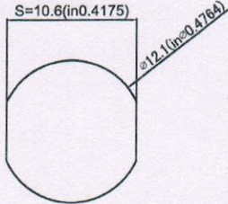
Panel hole size (面板开孔尺寸)
