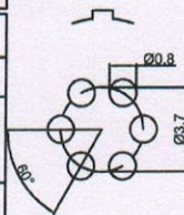
Pcb plate opening size (PCB板开孔尺寸)
