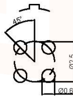
Pcb plate opening size (PCB板开孔尺寸)
