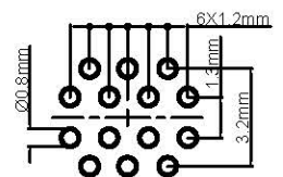
Pcb plate opening size (PCB板开孔尺寸)
