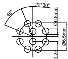
Pcb plate opening size (PCB板开孔尺寸)
