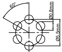
Pcb plate opening size (PCB板开孔尺寸)
