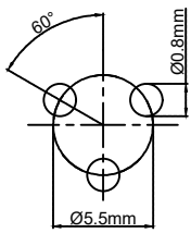
Pcb plate opening size (PCB板开孔尺寸)
