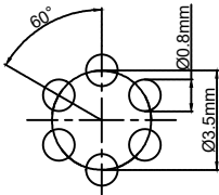
Pcb plate opening size (PCB板开孔尺寸)
