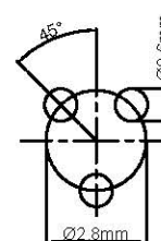
Pcb plate opening size (PCB板开孔尺寸)
