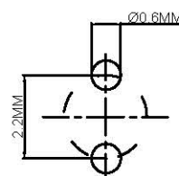
Pcb plate opening size (PCB板开孔尺寸)
