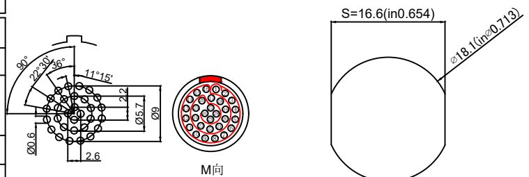
Pcb plate opening size (PCB板开孔尺寸)
