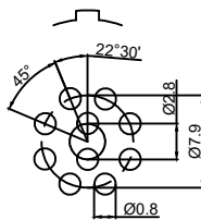
Pcb plate opening size (PCB板开孔尺寸)
