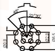
Pcb plate opening size (PCB板开孔尺寸)
