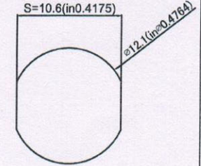
Pane hole size (面板开孔尺寸)
