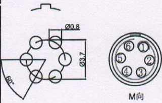
Pcb plate opening size (PCB板开孔尺寸)
