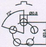
Pcb plate opening size (PCB板开孔尺寸)
