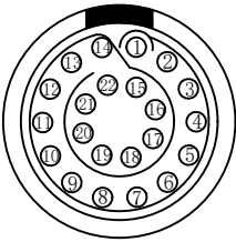
Welded surface (焊接面)
