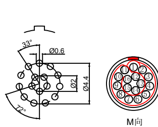
Pcb plate opening size (PCB板开孔尺寸)
