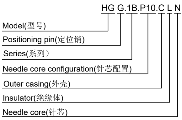
Boarded mother adhesive core (板接型母胶芯)
