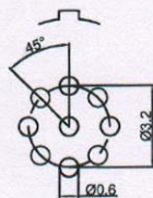
Pcb plate opening size (PCB板开孔尺寸)
